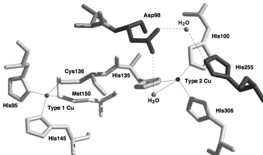
FIGURE 4. Type 1 and type 2 Cu sites in oxidized AxgNIR. The numbers refer to the AciNIR sequence. His306 residue comes from an adjacent subunit.
